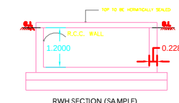
RWH_CAPACITY_L=2000LTRS
