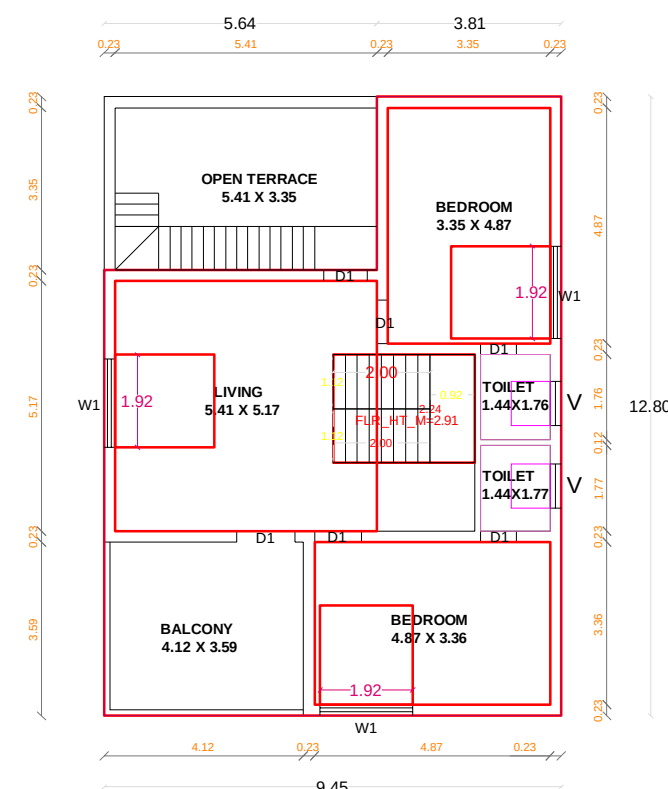
FIRST FLOOR PLAN PROPOSED
