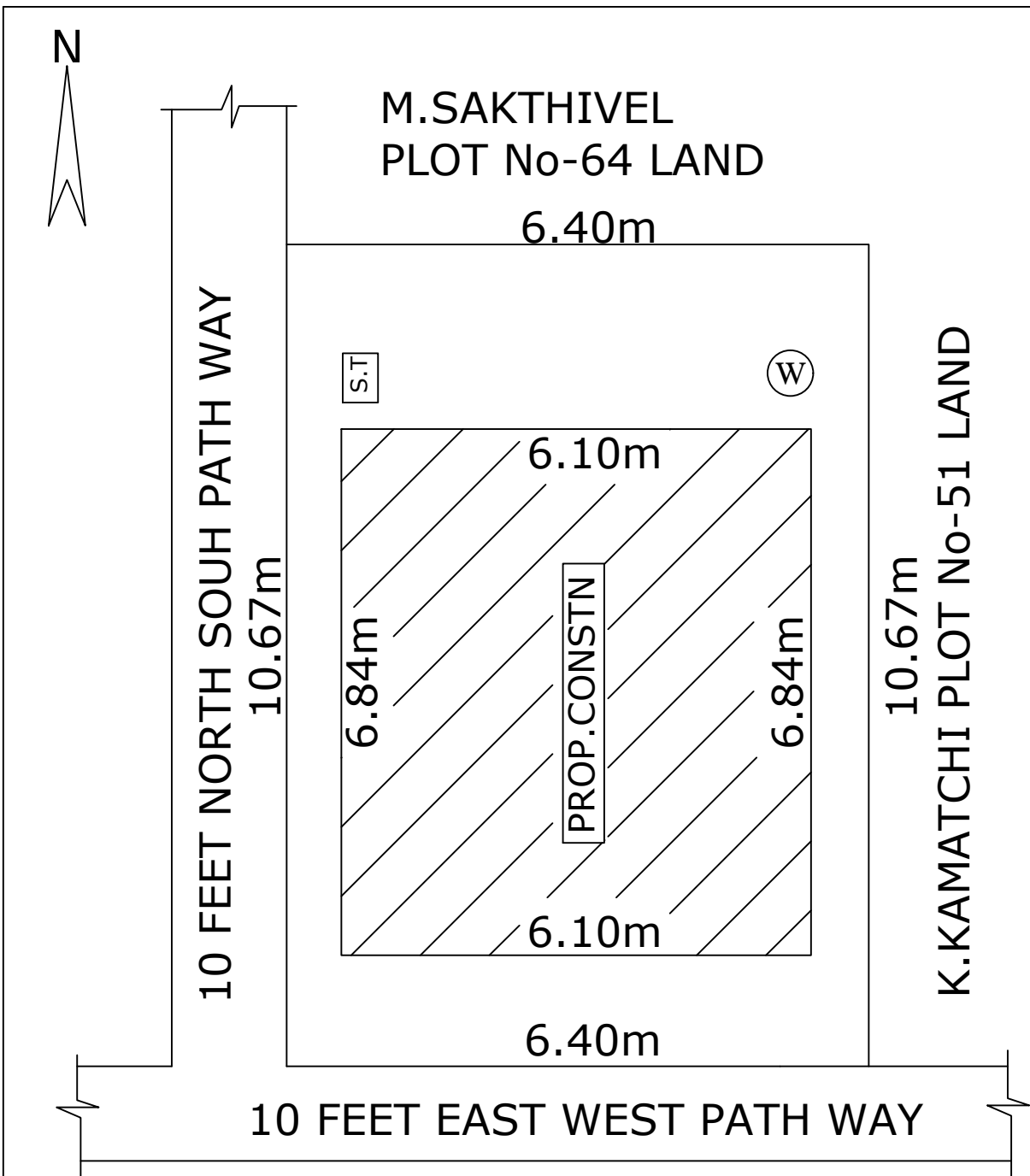
SITE PLAN
