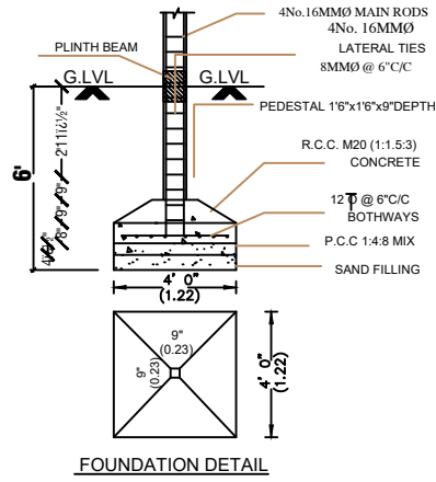
FOUNDATION DETAIL
