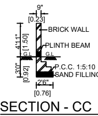
FOUNDATION DETAIL
