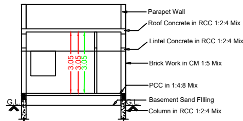
Section RR
