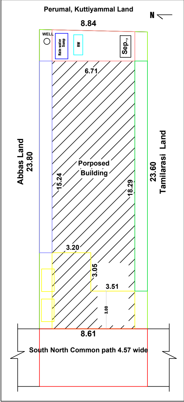
SITE PLAN CUM KEYPLAN
