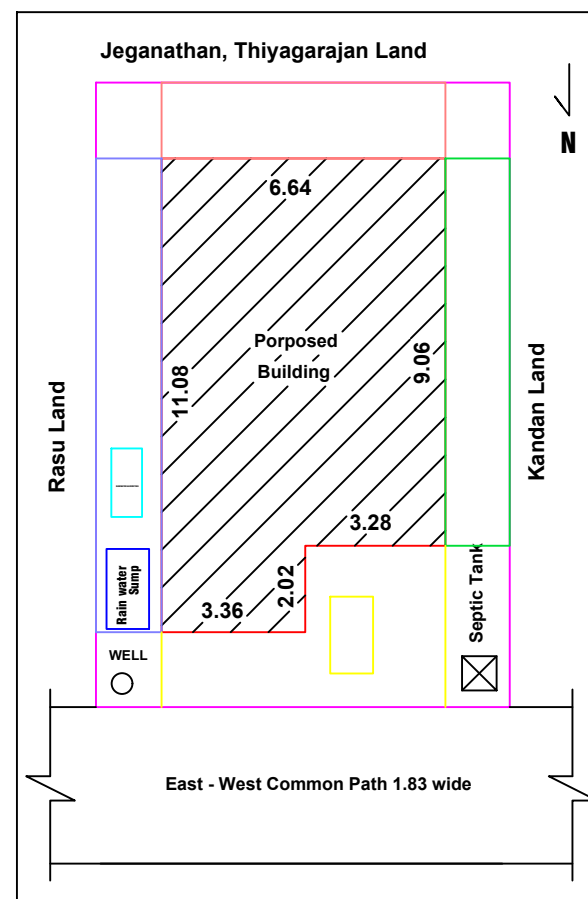
SITE PLAN CUM KEYPLAN
