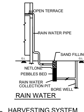
RAIN WATER HARVESTING SYSTEM
