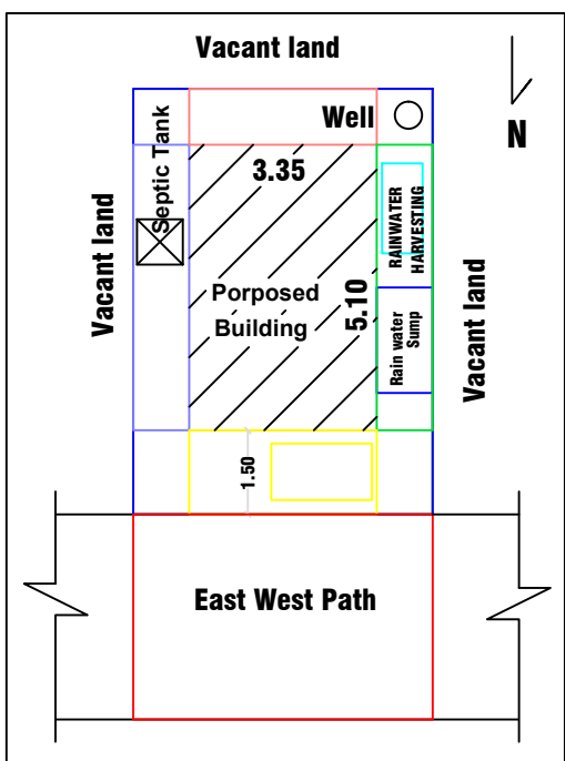
SITE PLAN CUM KEYPLAN
