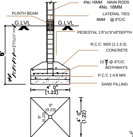
FOUNDATION DETAIL
