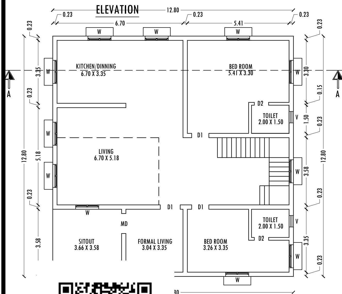
FLOOR PLAN
