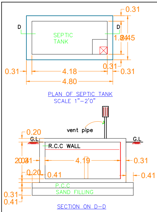
SECTION ON D-D
