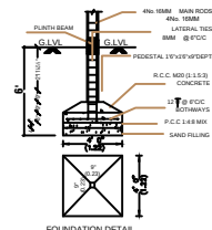
FOUNDATION DETAIL
