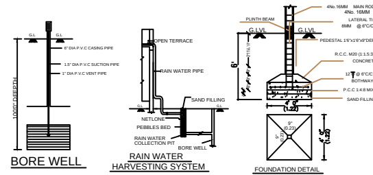
FOUNDATION DETAIL
