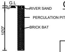
PERCULATION PIT
