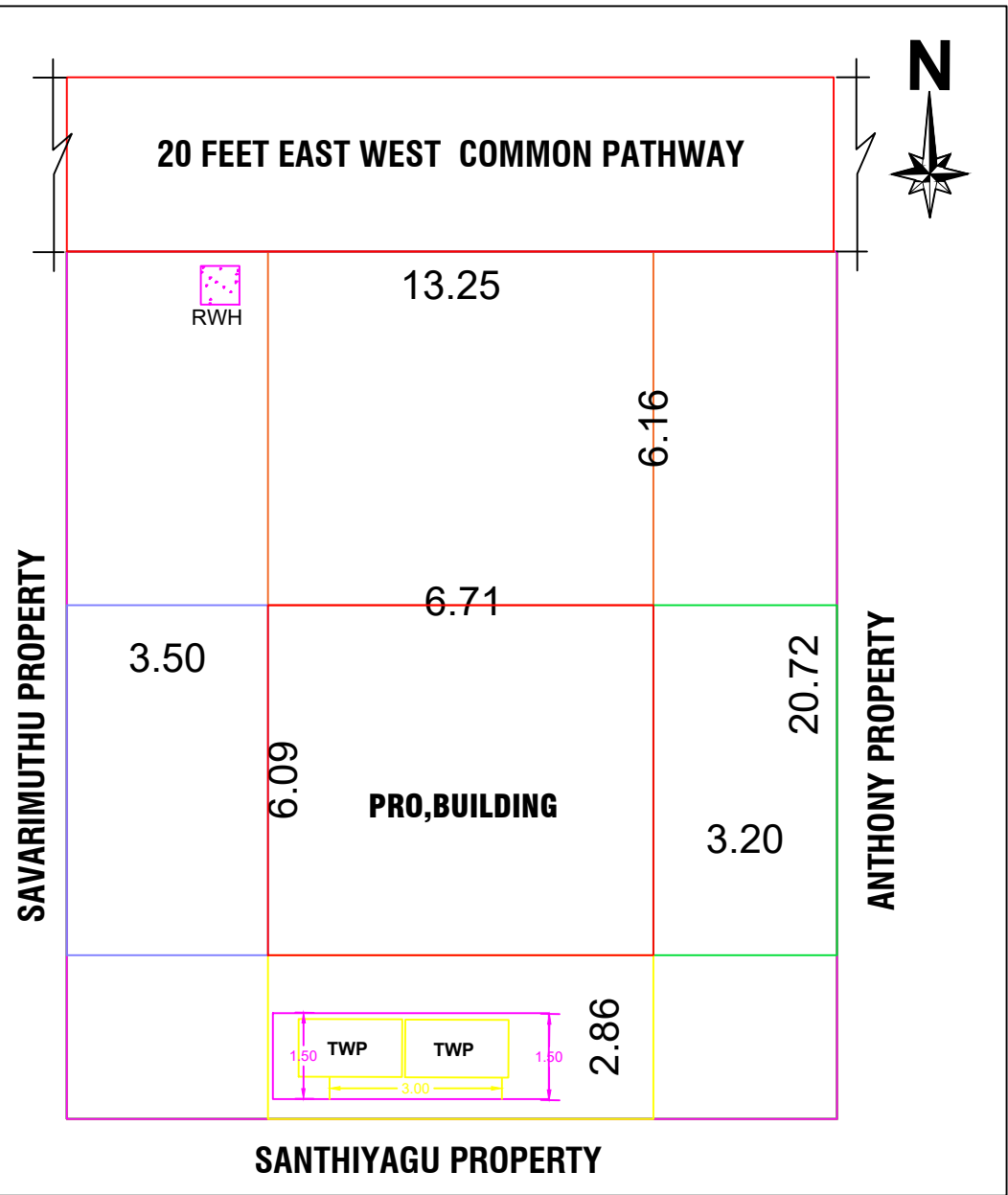
SITE PLAN
