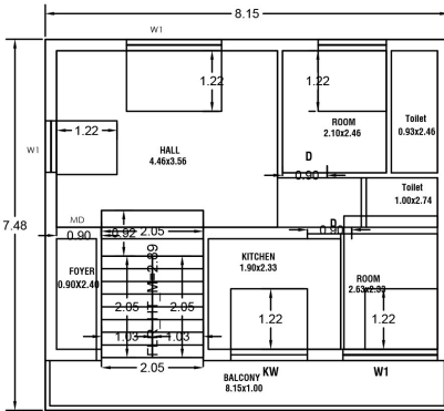
PRO., SECOND FLOOR PLAN HOUSE 3
