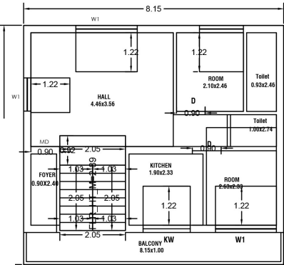
PRO., FIRST FLOOR PLAN HOUSE 2
