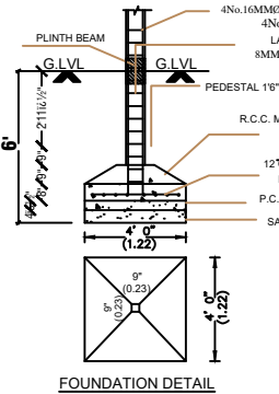
FOUNDATION DETAIL
