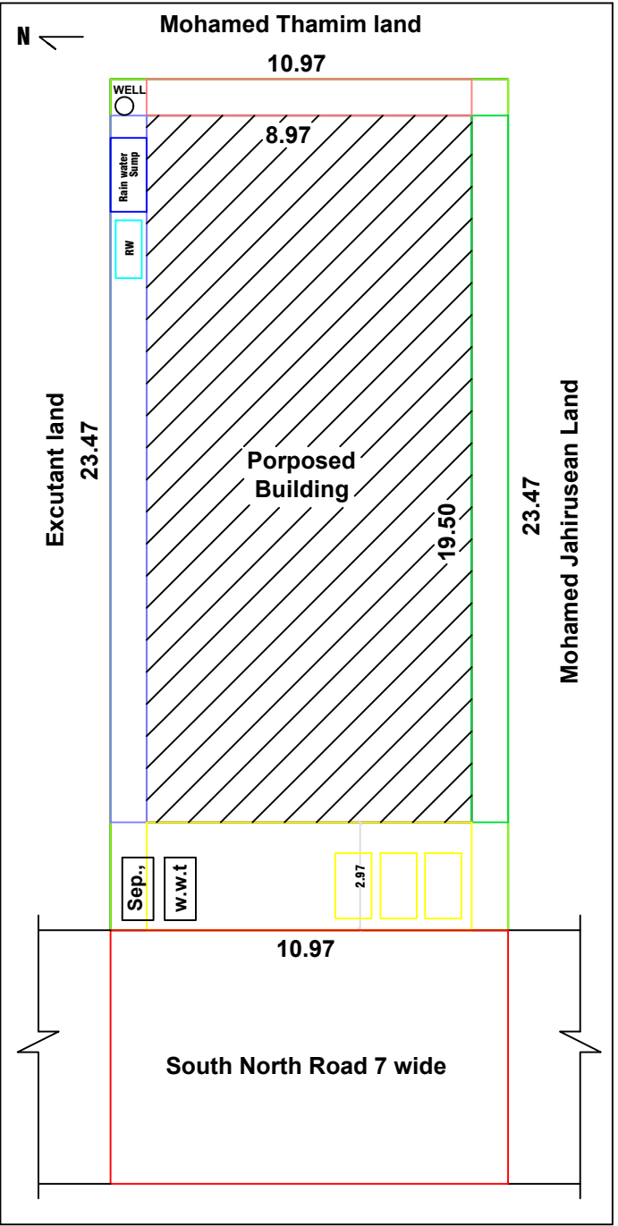
SITE PLAN CUM KEYPLAN
