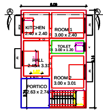
PROPOSED GROUND FLOOR
