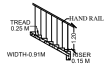
STAIRCASE DETAILS
