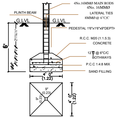
FOUNDATION DETAIL
