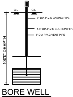
BORE WELL
