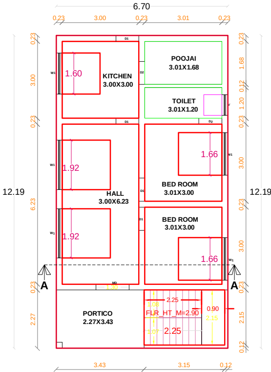
GROUND FLOOR PLAN PROPOSED
