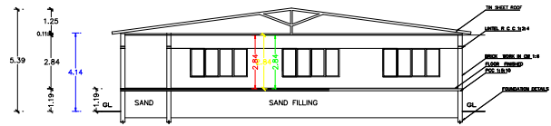
SECTION ON "A_B"
