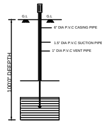
BORE WELL
