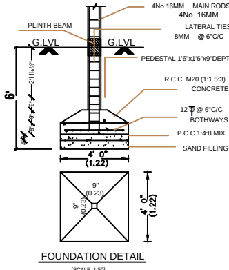
FOUNDATION DETAIL
