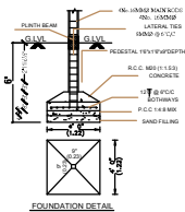
FOUNDATION DETAILS
