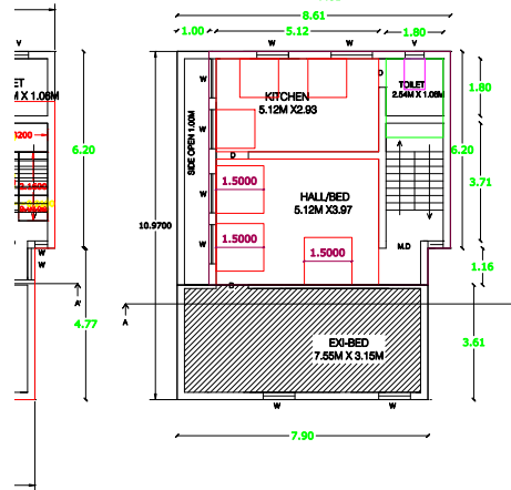
EXI & PRO- SECOND FLOOR PLAN
