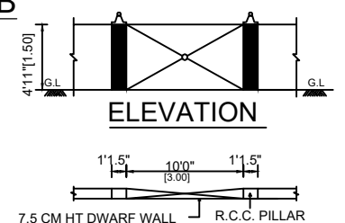
COMPOUND WALL PLAN
