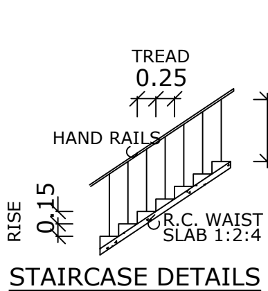
STAIRCASE DETAILS
