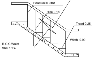
STAIRCASE DETAIL
