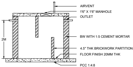
CROSS SECTION OF SEPTIC TANK
