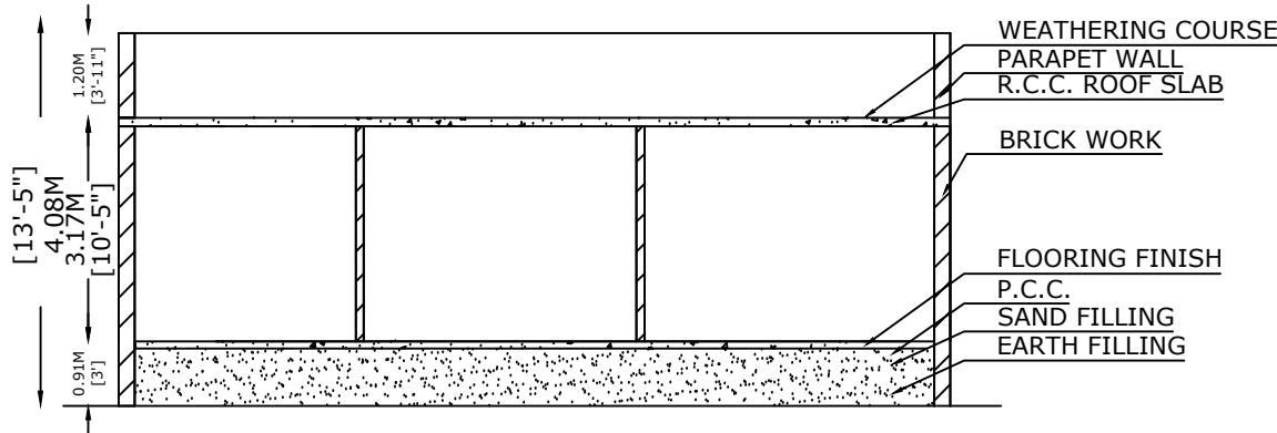
SECTION AN AA
