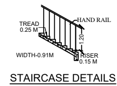
STAIRCASE DETAILS
