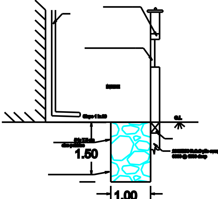
Percolation Pit
