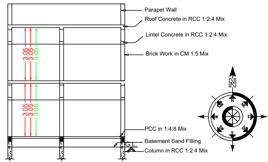
Section RR
