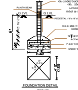
FOUNDATION DETAIL
