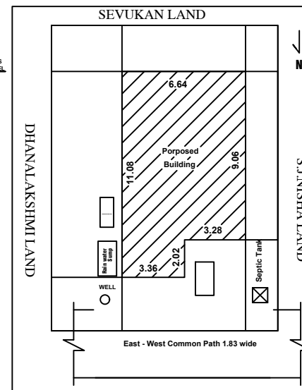
SITE PLAN CUM KEYPLAN
