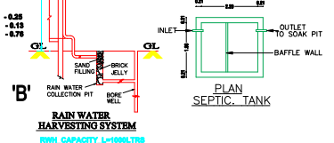
RAIN WATER HARVESTING SYSTEM
