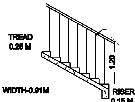
STAIRCASE DETAILS
