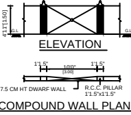
COMPOUND WALL PLAN
