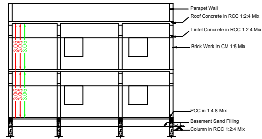
Section RR
