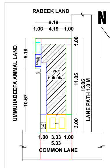
SITE PLAN & KEY PLAN
