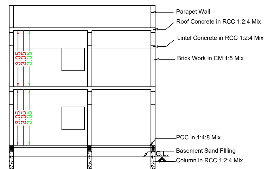
Section RR
