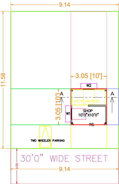
SITE CUM GROUND FLOOR
