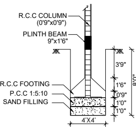
FOUNDATION DETAILS
