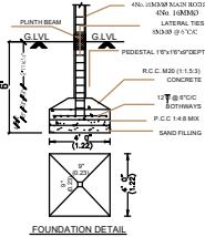
FOUNDATION DETAIL
