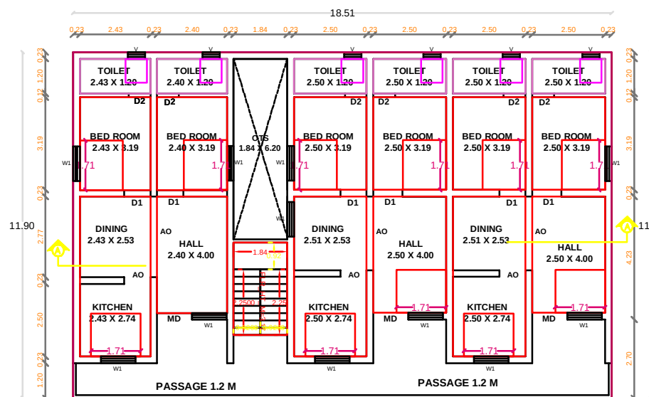
FIRST FLOOR PLAN PROPOSED
