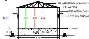
BLOCK 3 SECTION AB
