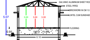
BLOCK 2 SECTION AB
