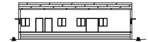
BLOCK 1 FRONT ELEVATION
