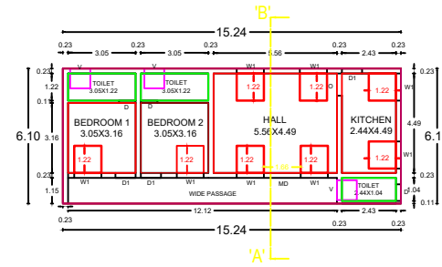
BLOCK 3 GROUND FLOOR PLAN PROPOSED
