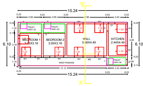
BLOCK 1 GROUND FLOOR PLAN PROPOSED
