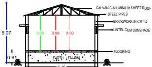
BLOCK 1 SECTION AB
