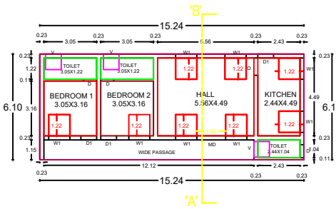
BLOCK 2 GROUND FLOOR PLAN PROPOSED
