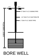
BORE WELL
