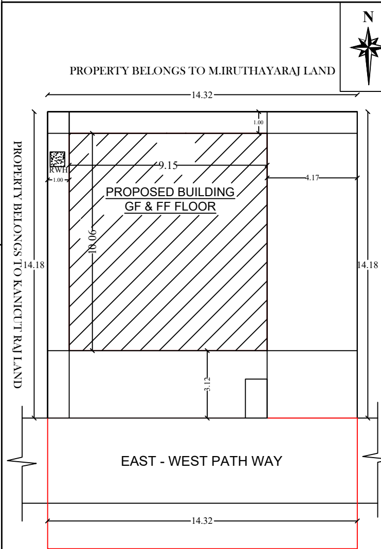
SITE PLAN
