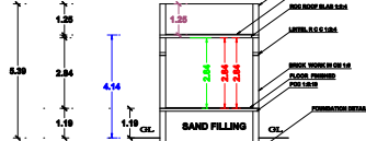
SECTION ON "A B"
