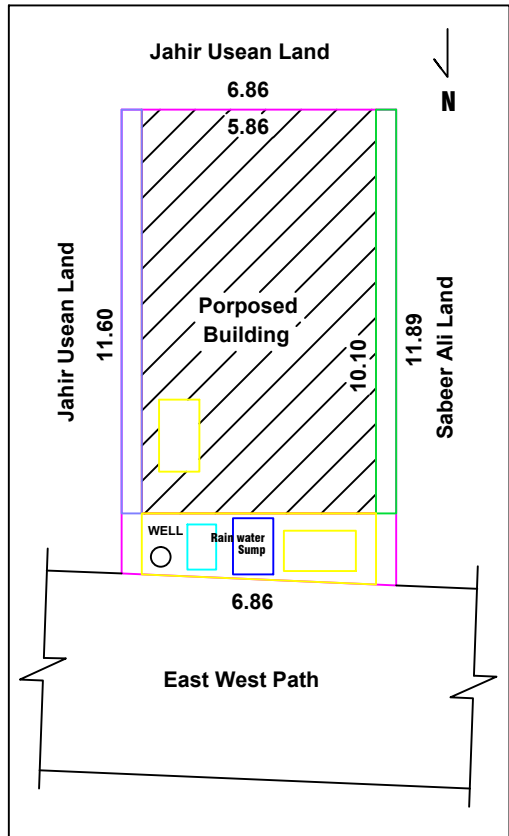
SITE PLAN CUM KEYPLAN
