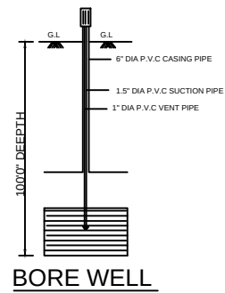
BORE WELL
