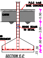
DETAILS OF COLUMN FOOTING
