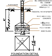
FOUNDATION DETAIL
