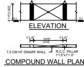
COMPOUND WALL PLAN
