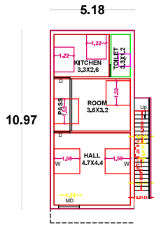
GROUND FLOOR I
