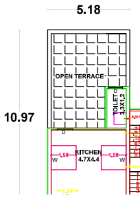
GROUND FLOOR II
