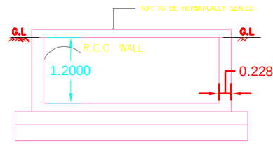
RWH SECTION (SAMPLE) RWH_CAPACITY_L=2000LTRS
