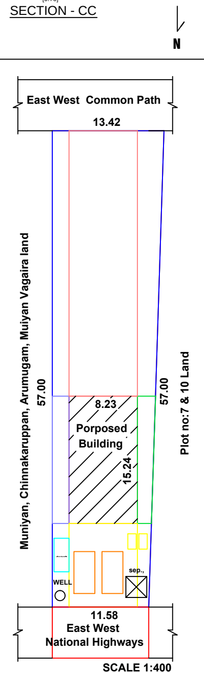
SITE PLAN CUM KEYPLAN
