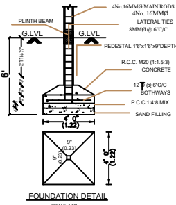
FOUNDATION DETAIL
