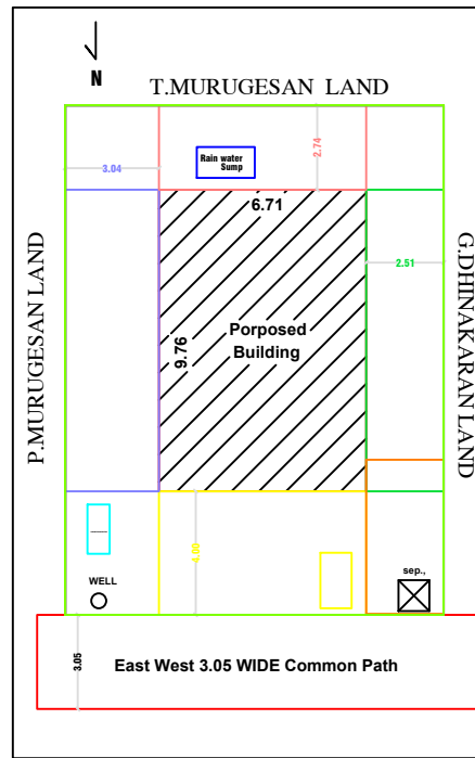
SITE PLAN CUM KEYPLAN
